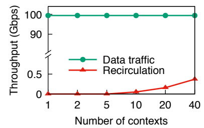
(c) Num. of contexts vs. traffic overhead
