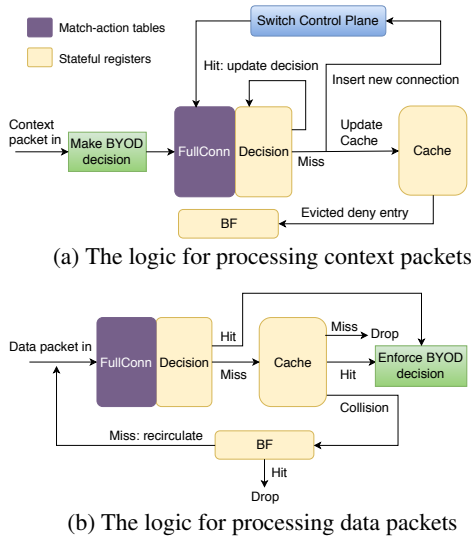
Figure 6: Poise uses a combination of match/action tables and stateful registers to process context and data packets.
