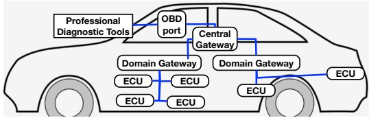
Figure 1: Communication system in the vehicle.
